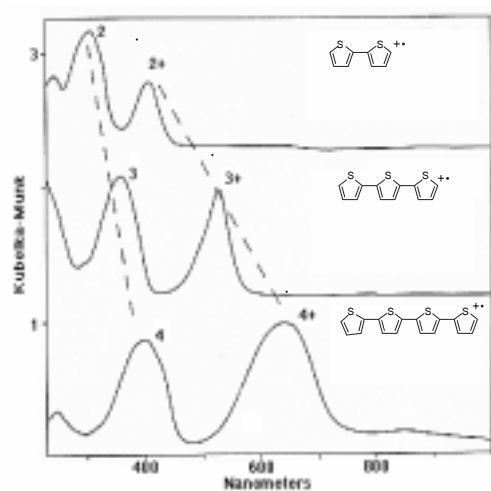
Figure 9: Radical cation formation of thiophene oligomers upon inclusion within Na + ZSM-5. Diffuse reflectance spectra of radical cations recorded at room temperature.
